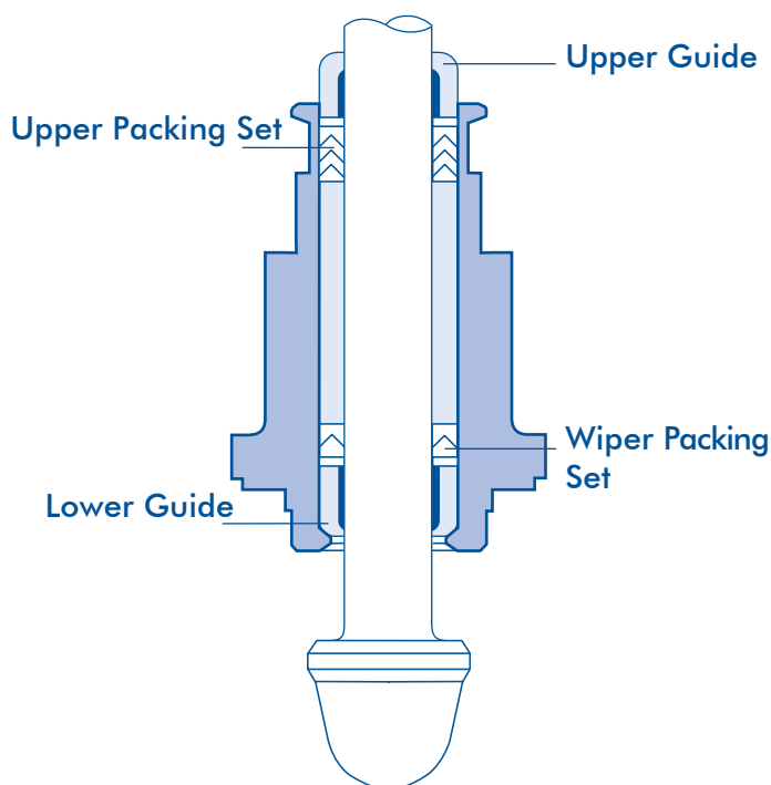
Figure 12: Typical Teflon V-ring Arrangement
