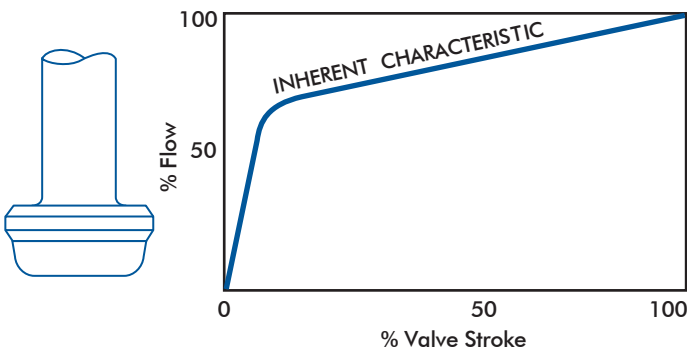
Figure 13: Flow Characteristics
